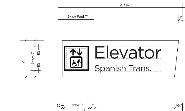
2 FRONT VIEW SCALE: 1 - 1/2" = 1' - 0"
