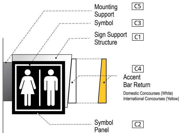
6 SIGN FINISHES SCALE: NTS
