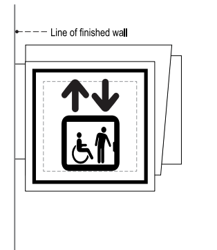
3 FRONT VIEW - ELEVATOR SCALE: 1-1/2" = 1' - 0"
