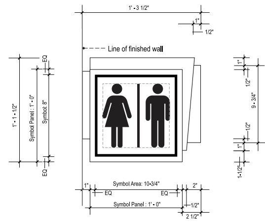
2 FRONT VIEW - RESTROOMS SCALE: 1-1/2" = 1' - 0"
