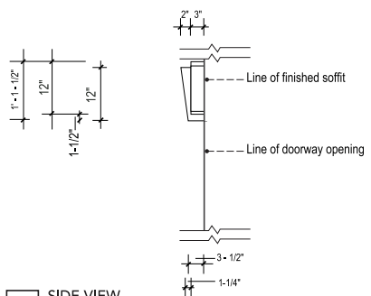
3 SIDE VIEW SCALE: 1/2" = 1' - 0"
