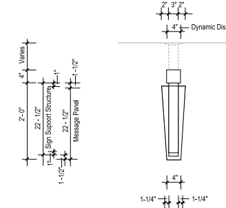
3 SIDE VIEW SCALE: 1/2" = 1' - 0"
