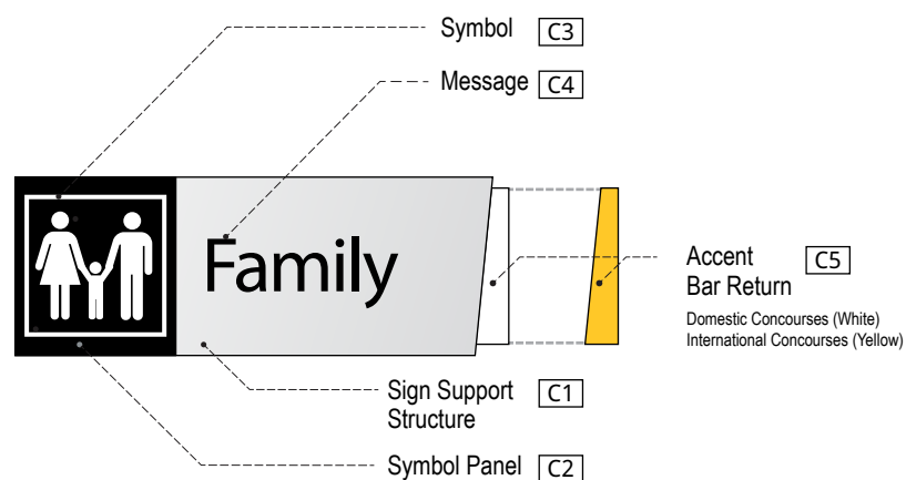
7 SIGN FINISHES SCALE: NTS
