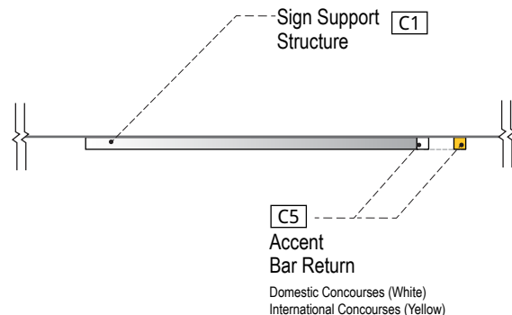
8 TOP VIEW SIGN FINISHES SCALE: NTS
