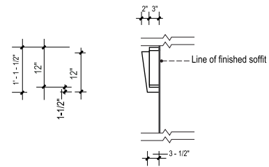
3 SIDE VIEW SCALE: 1/2" = 1' - 0"
